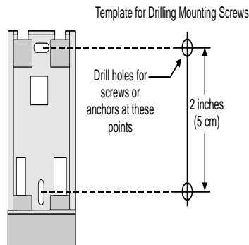
Figure 15 Bracket Template
